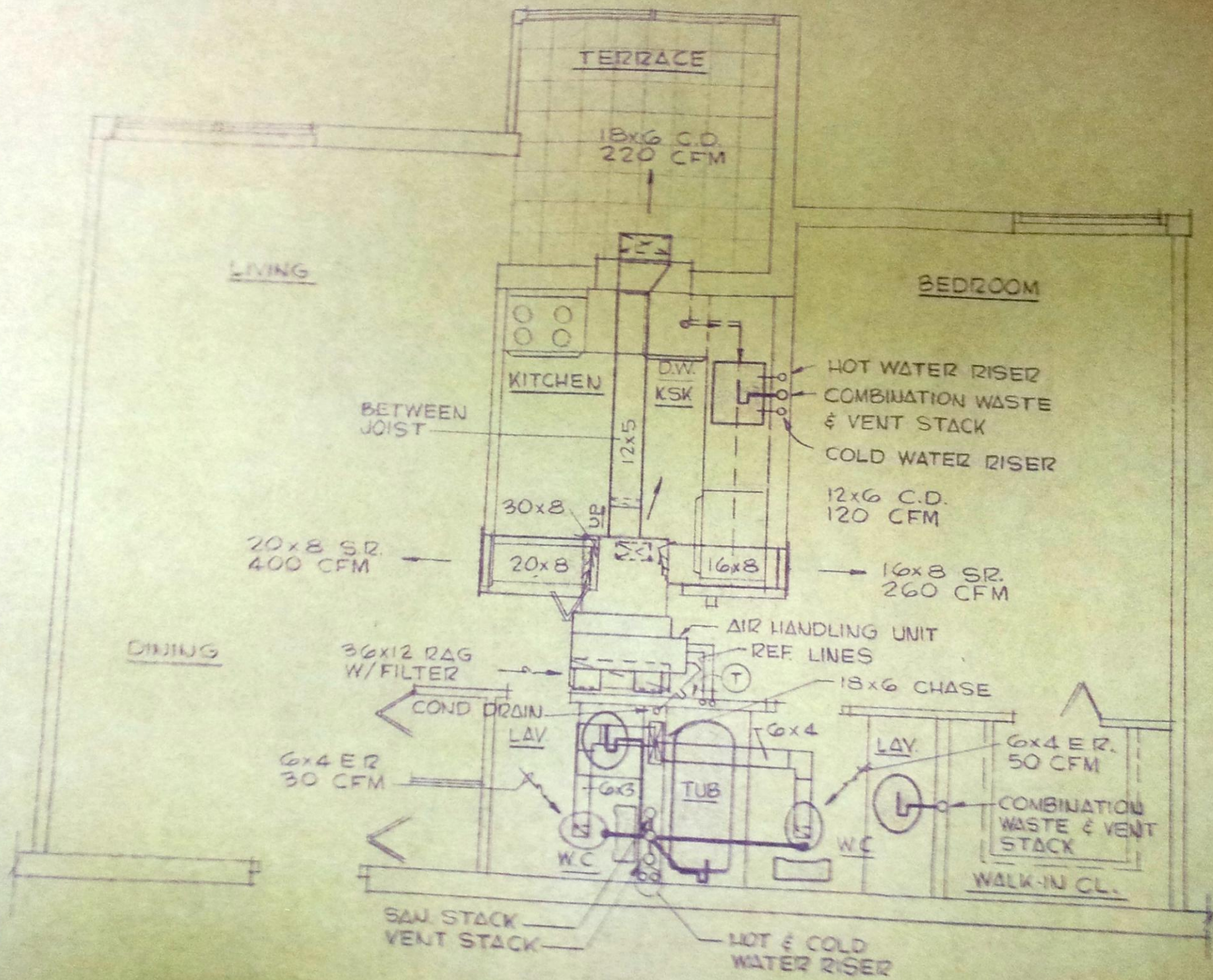
APARTMENT TYPE 'A' FLOOR PLAN SCALE 1/8" = 1'-0"
